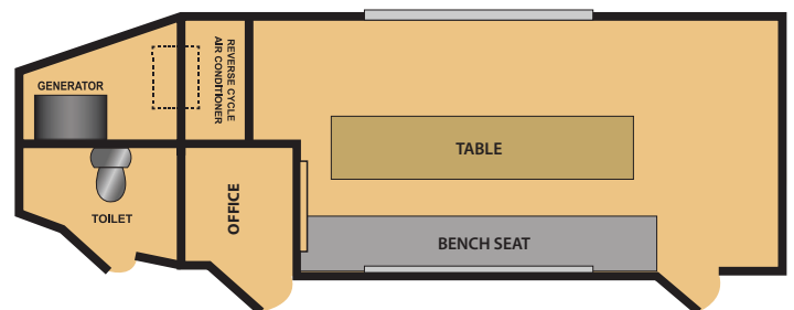
MTELO Floorplan
