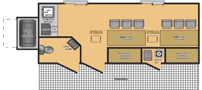
MT1 Floorplan
